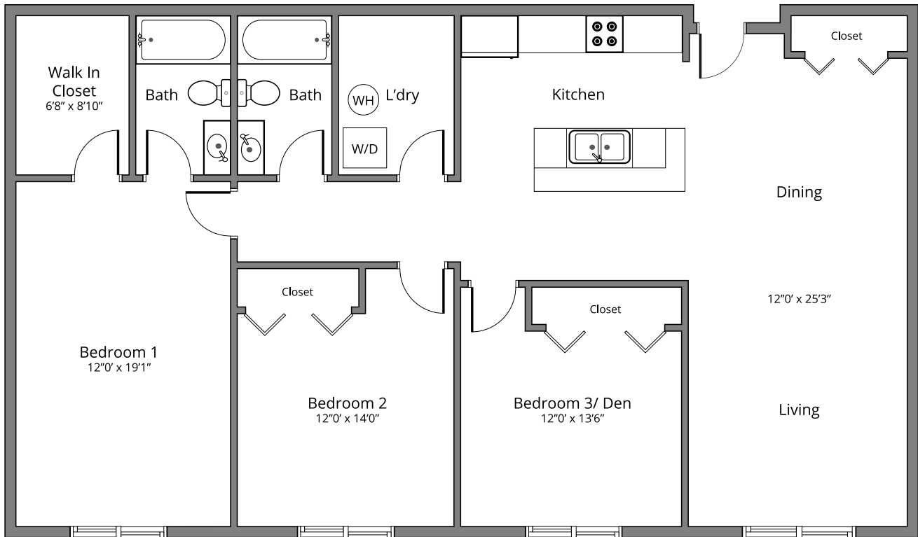
THREE BEDROOM PLAN
